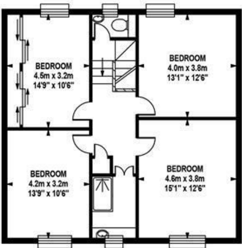
FIRST FLOOR Approximate Internal Area :- 77.39 sq m / 833 sq ft
