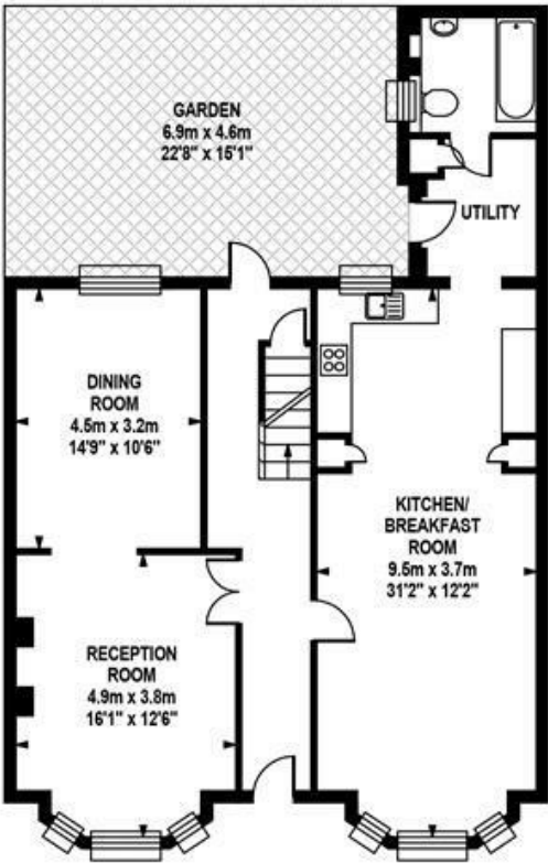
GROUND FLOOR Approximate Internal Area :- 91.79 sq m / 988 sq ft
